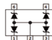
Schematic Symbol
