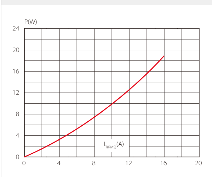
FIG.1 Maximum power dissipation versus RMS on-state current
