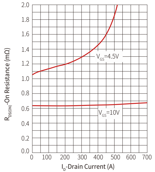
Figure 6: On Resistance
