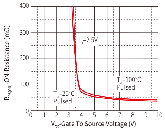
Figure 4: R_{DS(ON)} — V_{GS}
