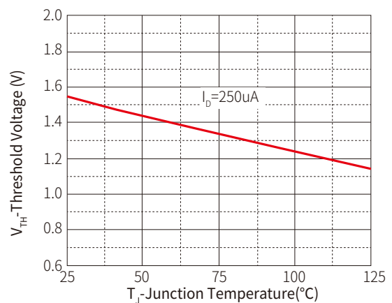
Figure 6: Threshold Voltage
