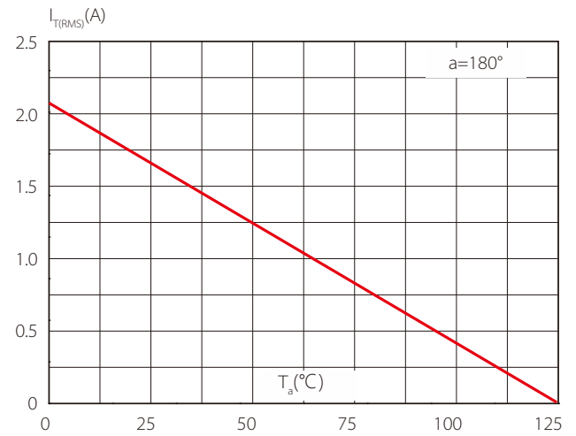
FIG.2: RMS on-state current versus ambient temperature (printed circuit board FR4, copper thickness: 35μm)
