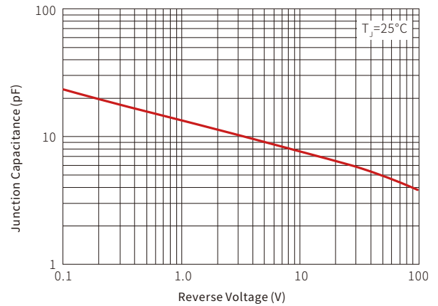
Fig. 4-Typical Junction Capacitance
