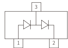
Schematic Symbol
