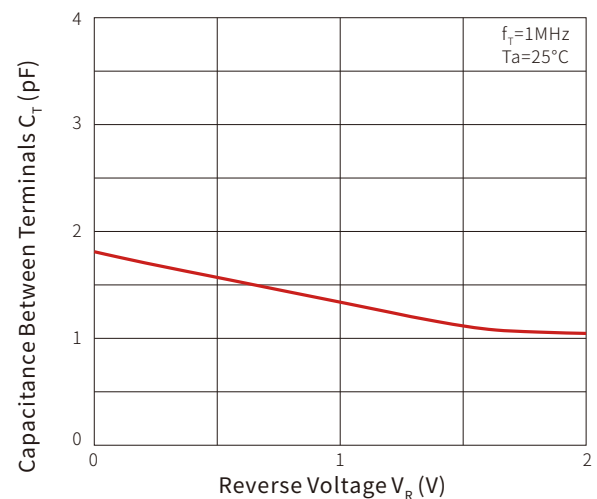
Fig 2. Capacitance Capability
