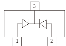
Schematic Symbol
