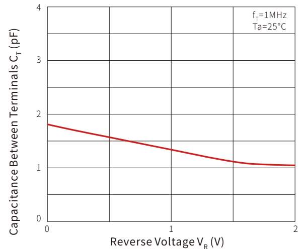
Fig 2. Capacitance Capability
