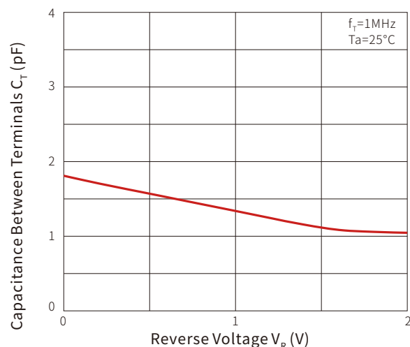
Fig 2. Capacitance Capability
