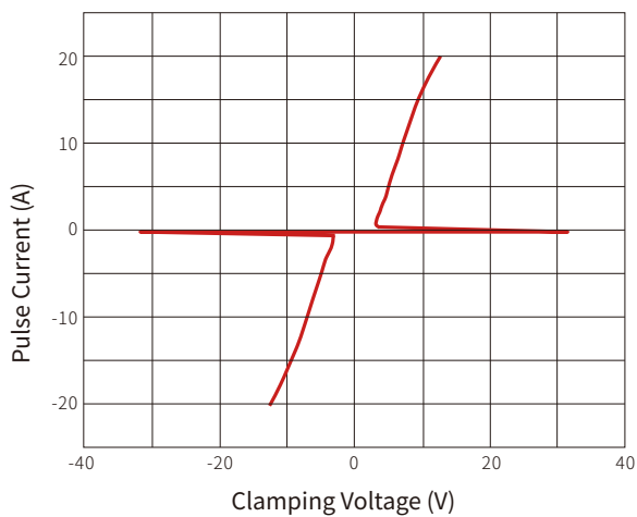
Transmission Line Pulse Curve
