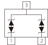
Schematic Symbol
