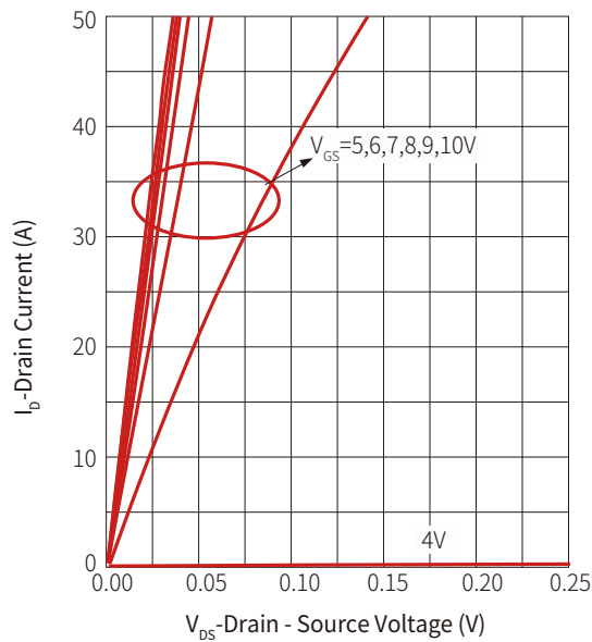
Figure 5: Output Characteristics
