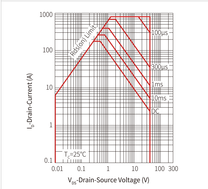
Figure3: Safe operating Area
