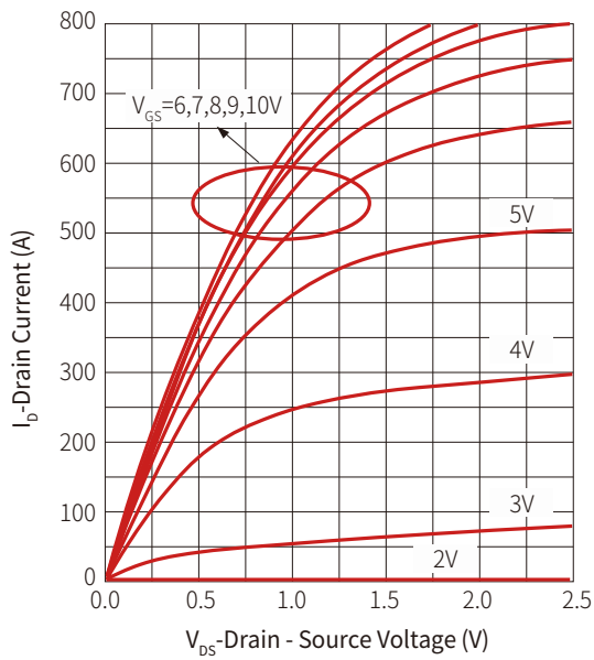
Figure 5: Output Characteristics
