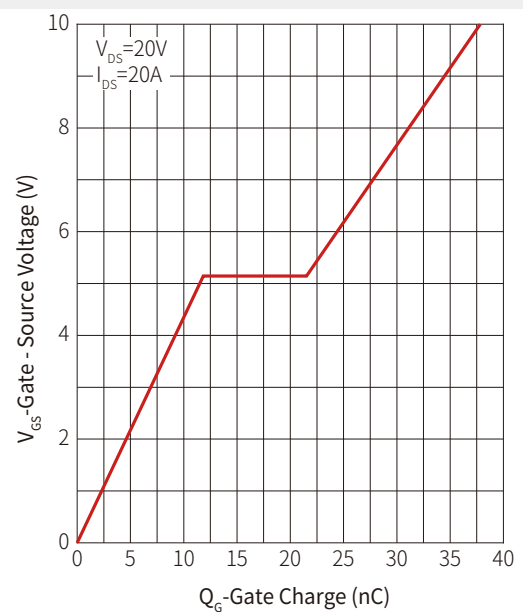
Figure 12: Gate Charge
