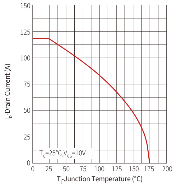
Figure2: Current Capability
