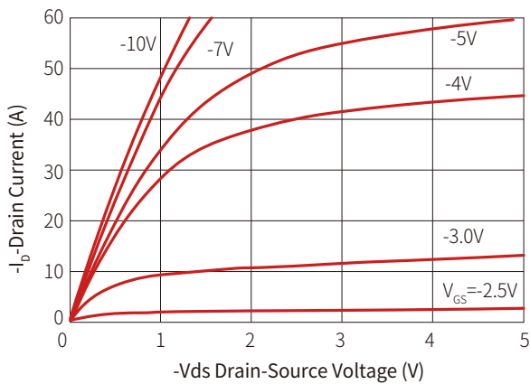
Figure 1: Output Characteristic
