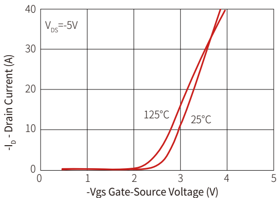
Figure 3: Transfer Characteristic
