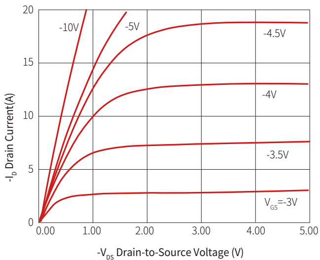
Figure1: Output Characteristic
