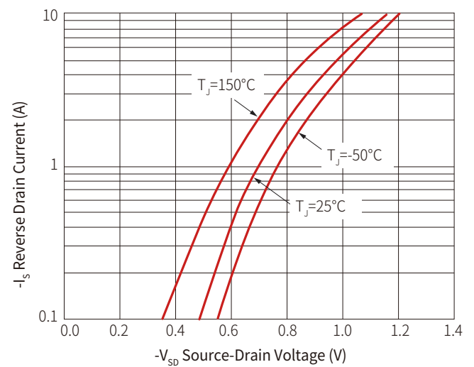
Figure 8: Body Diode Characteristic
