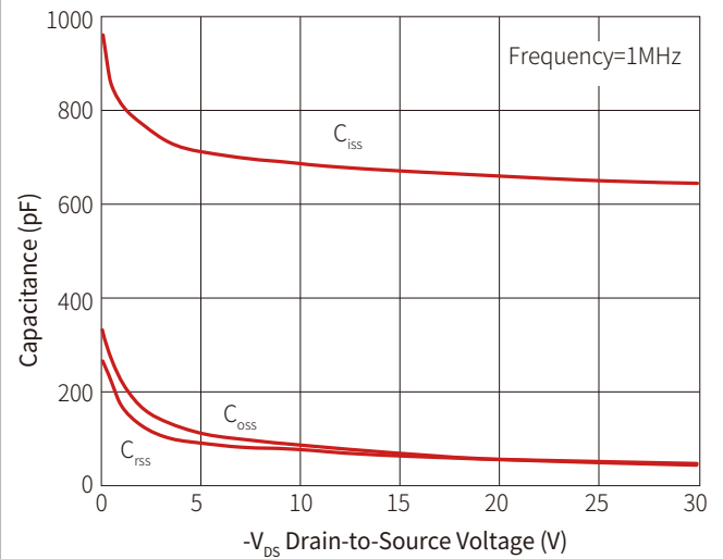
Figure 6: Capacitance Characteristic
