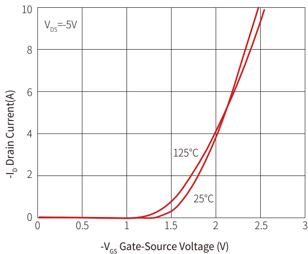
Figure3: Transfer Characteristic
