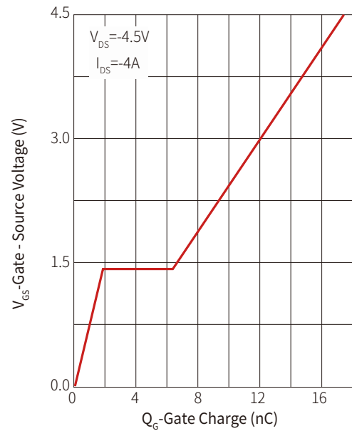
Figure 12: Gate Charge
