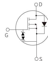
Schematic Symbol
