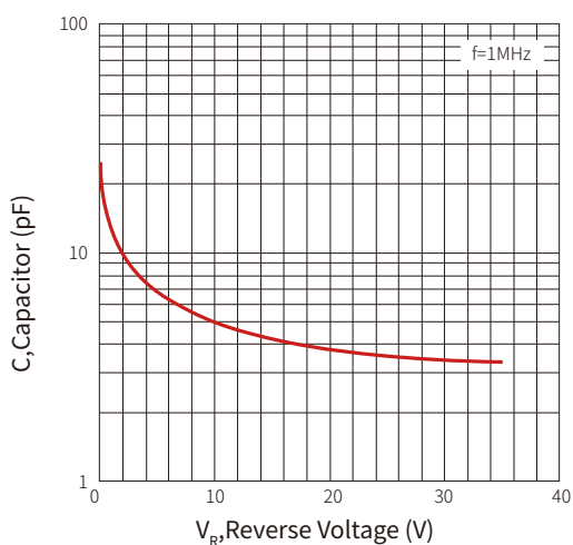
Fig.3 Capacitor Characteristics
