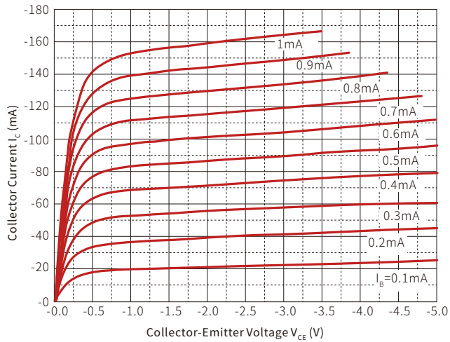
Static Characteristic
