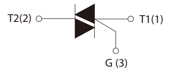
Schematic Symbol
