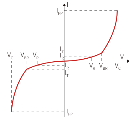
Figure 1: V- I curve characteristics (Bi-directional)
