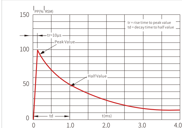
Figure 3: Pulse waveform
